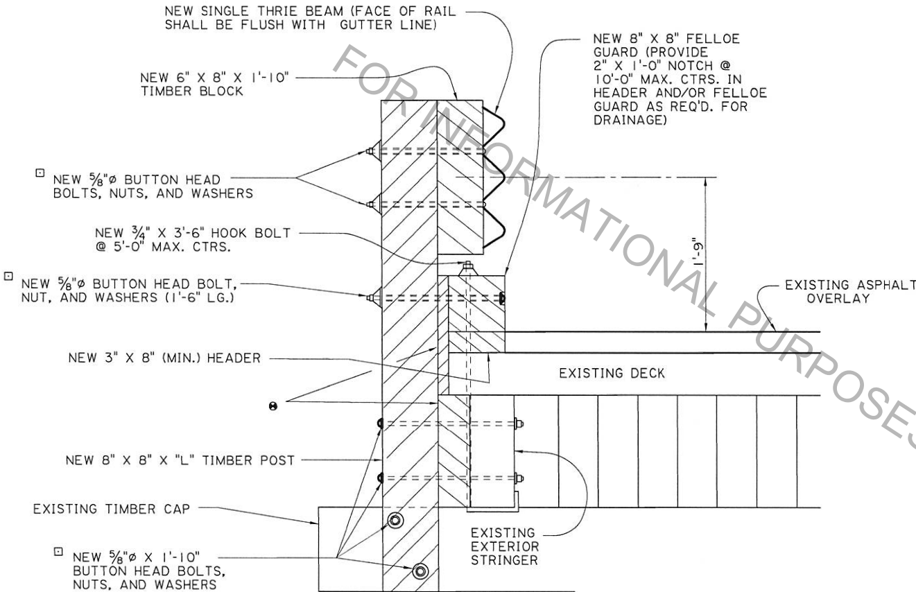
TYPICAL SECTION
